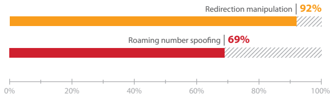
Figure 11. Percentage of successful attacks in order to redirect a terminating call by method
